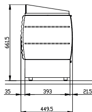
Schaerer Coffee Celebration W Tassenwärmer Cup warmer
