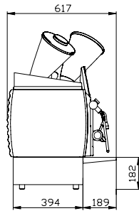
Schaerer Coffee Celebration BCL Kaffee, Heisswasser, Dampf, Milch Coffee, hot water, steam, milk
